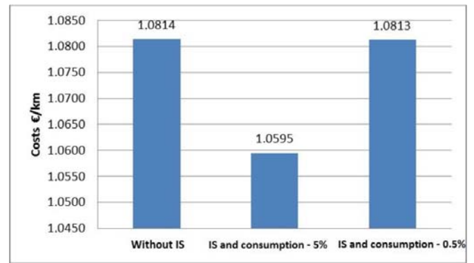
Figure 1. – Comparison of costs in €/km within the fuel consumption reduction
