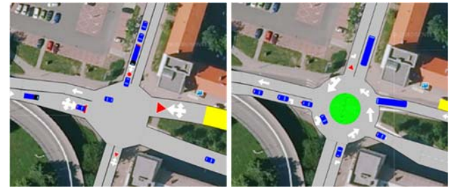
Figure 4. Creation of transport models for current and future state, source: author - processed in Aimsun software
